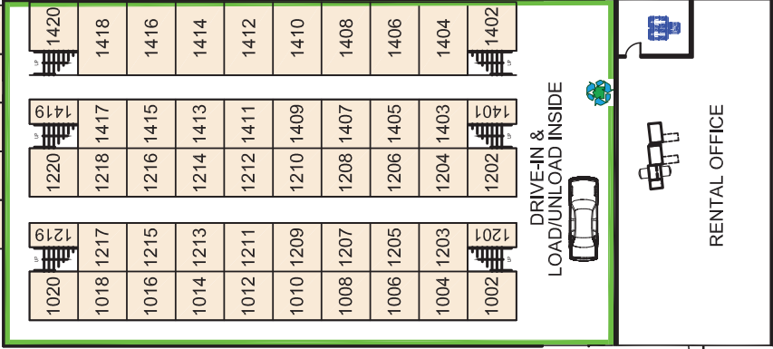
BUILDING A - LOWER LEVEL
