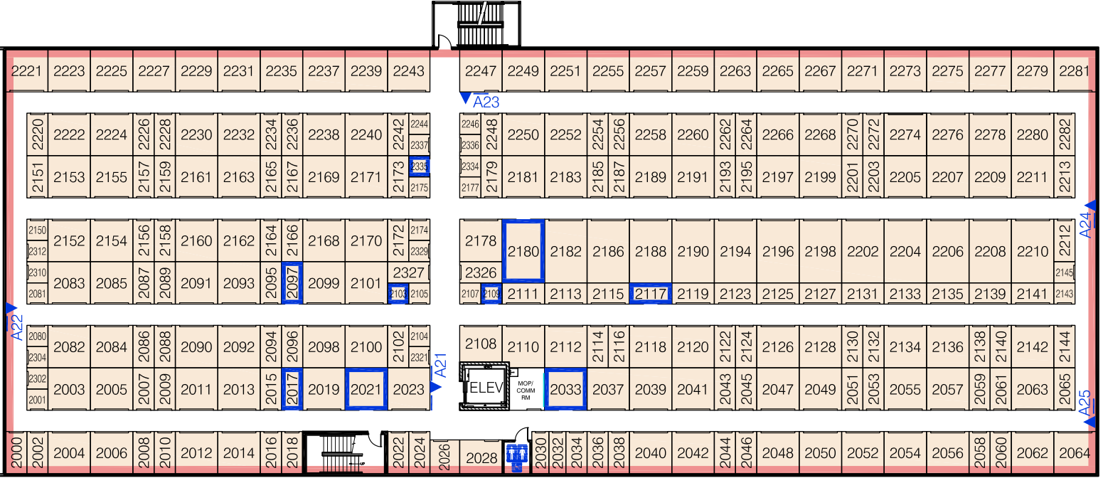
SECOND FLOOR
