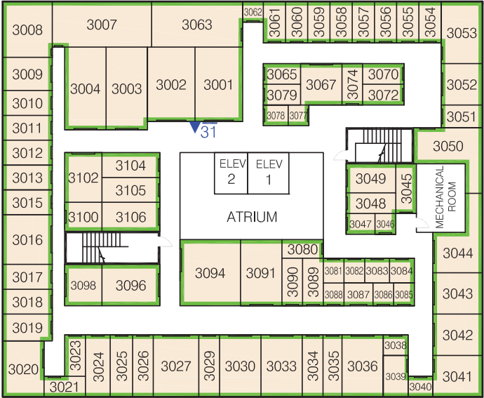
BUILDING A- THIRD FLOOR
