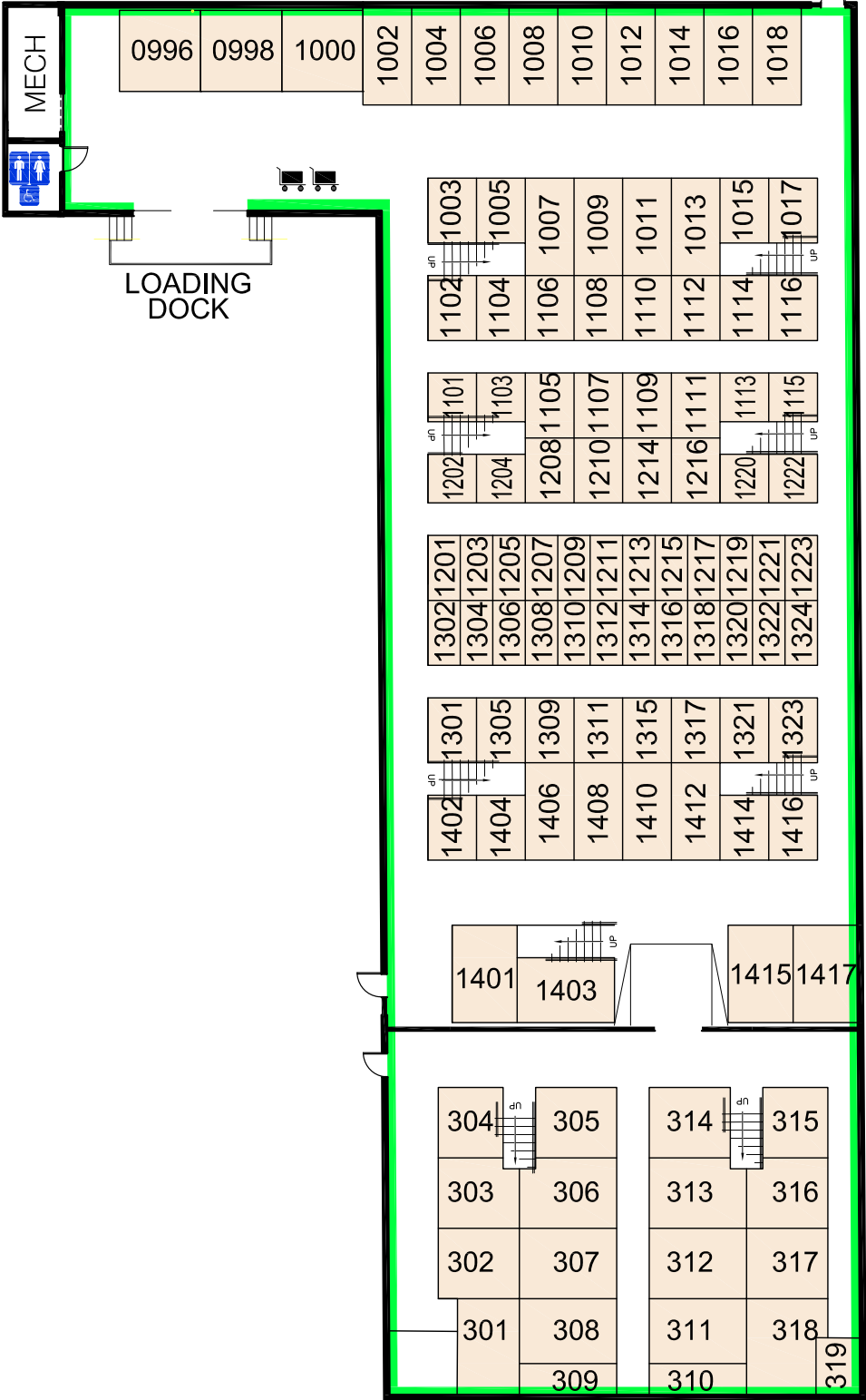
BUILDING B - FIRST FLOOR
