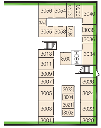
BUILDING A - SECOND FLOOR
