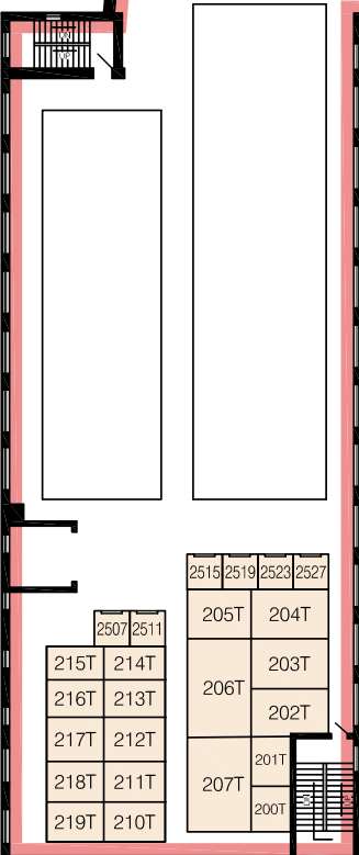
SECOND FLOOR - UPPER LEVEL
