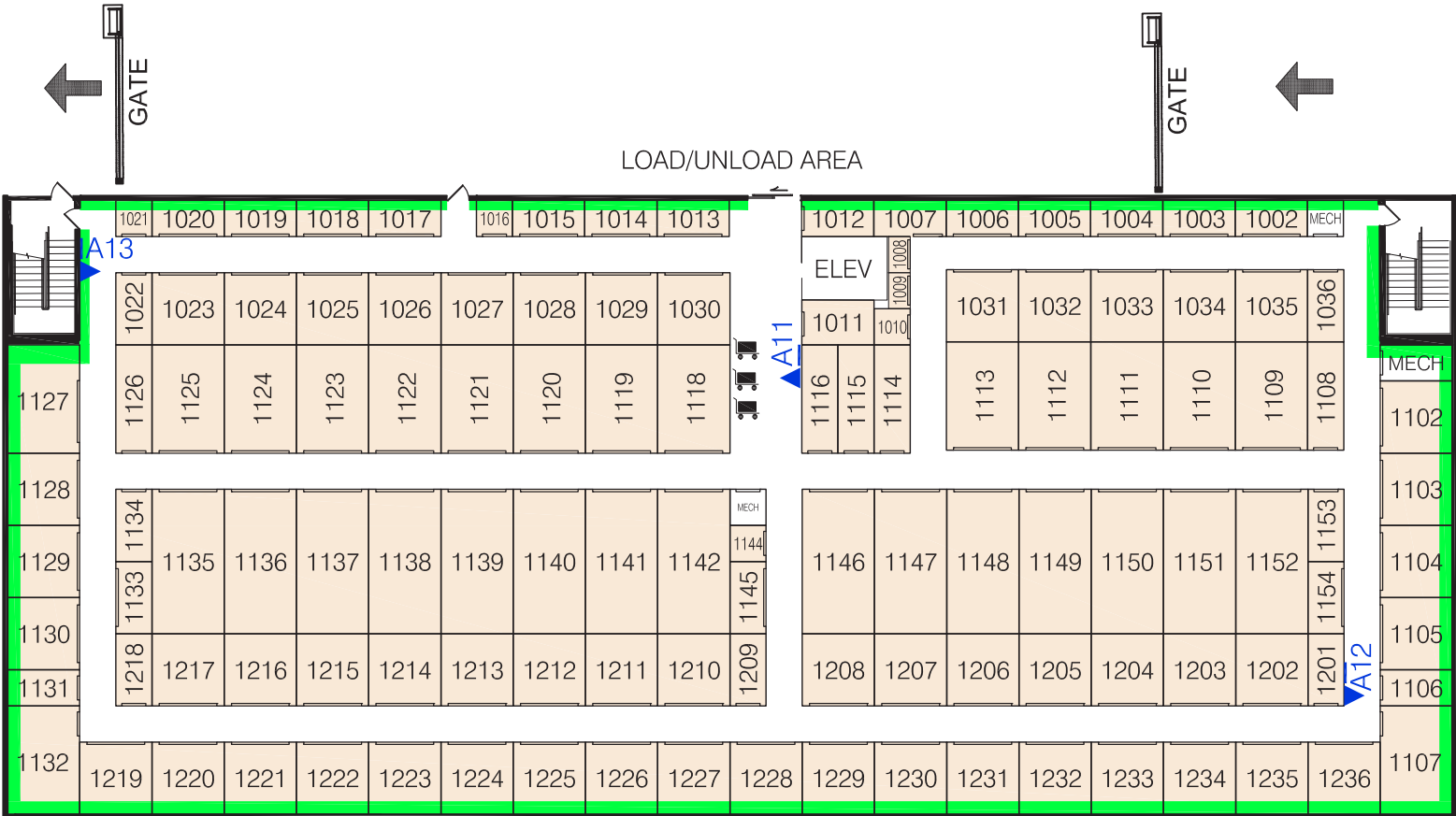
FIRST FLOOR
