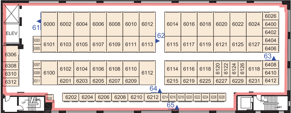
SIXTH FLOOR
