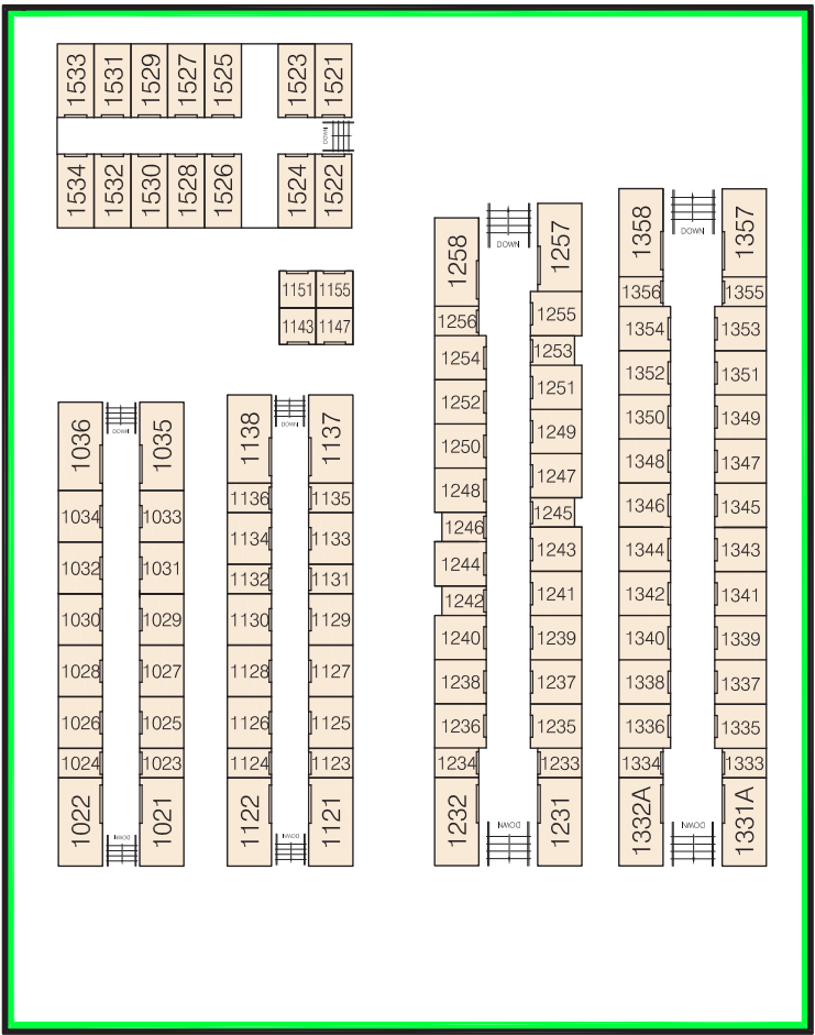
FIRST FLOOR- UPPER LEVEL
