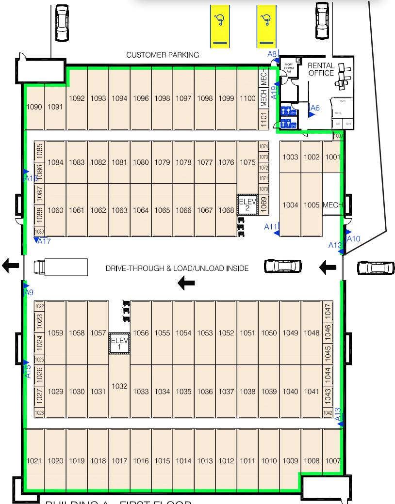
BUILDING A - FIRST FLOOR
