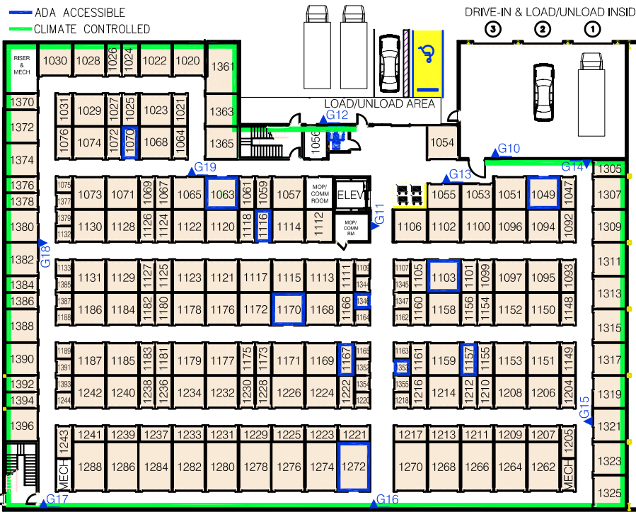
BUILDING G - FIRST FLOOR
