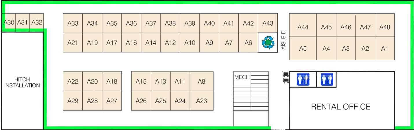
FIRST FLOOR
