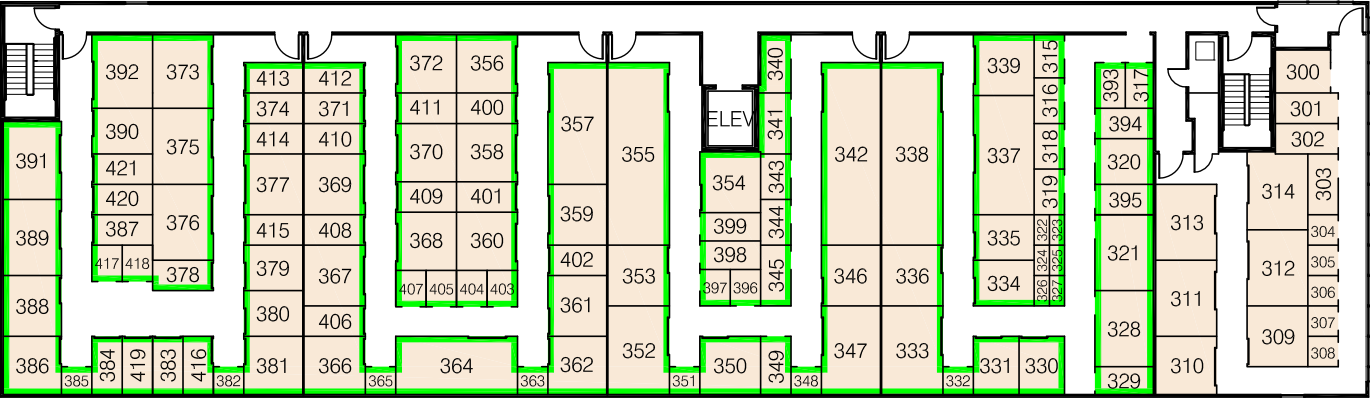
BUILDING B - THIRD FLOOR
