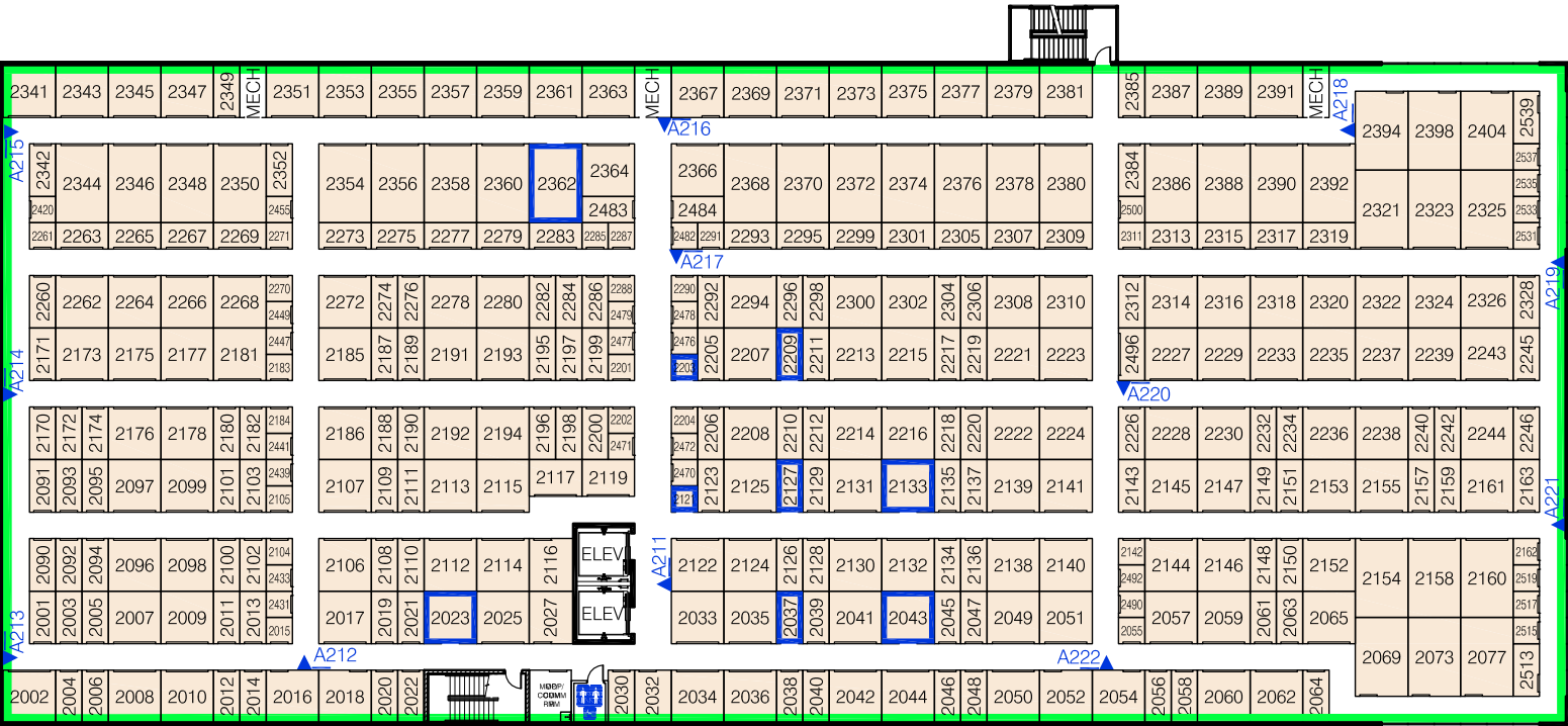
BUILDING A - SECOND FLOOR
