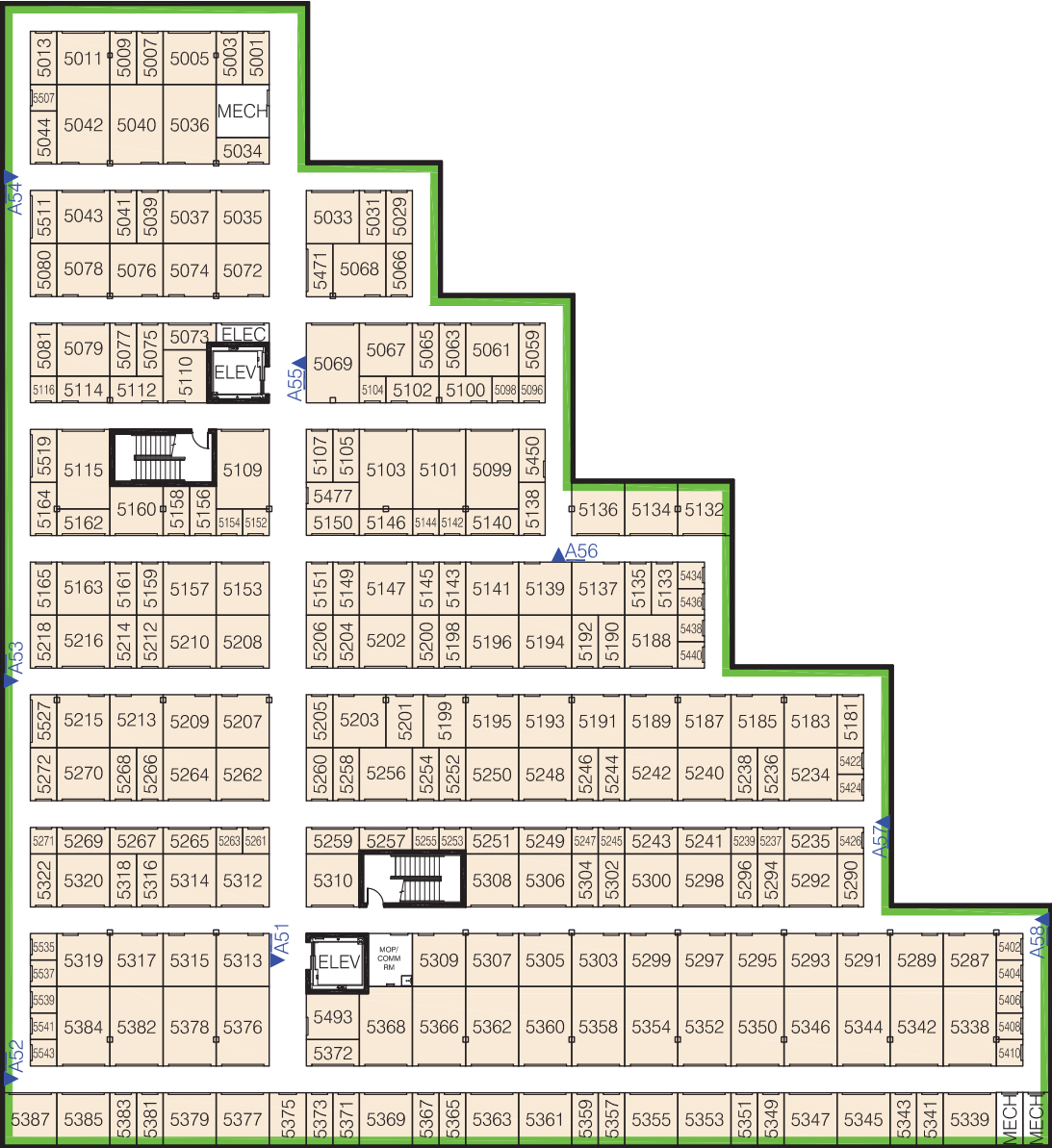
BUILDING A - FIFTH FLOOR
