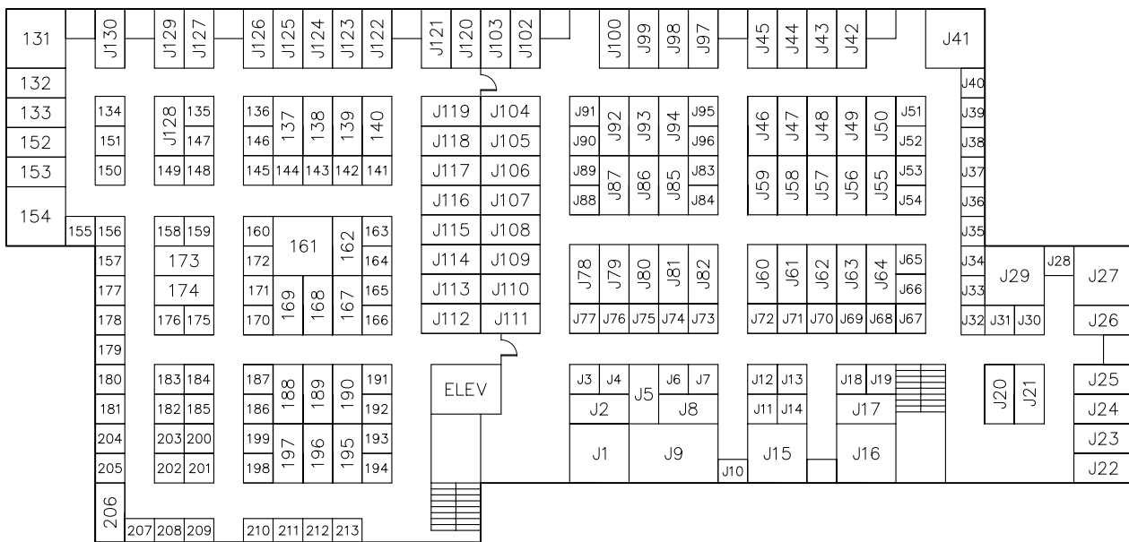
BLDG - 'J' SECOND FLOOR
