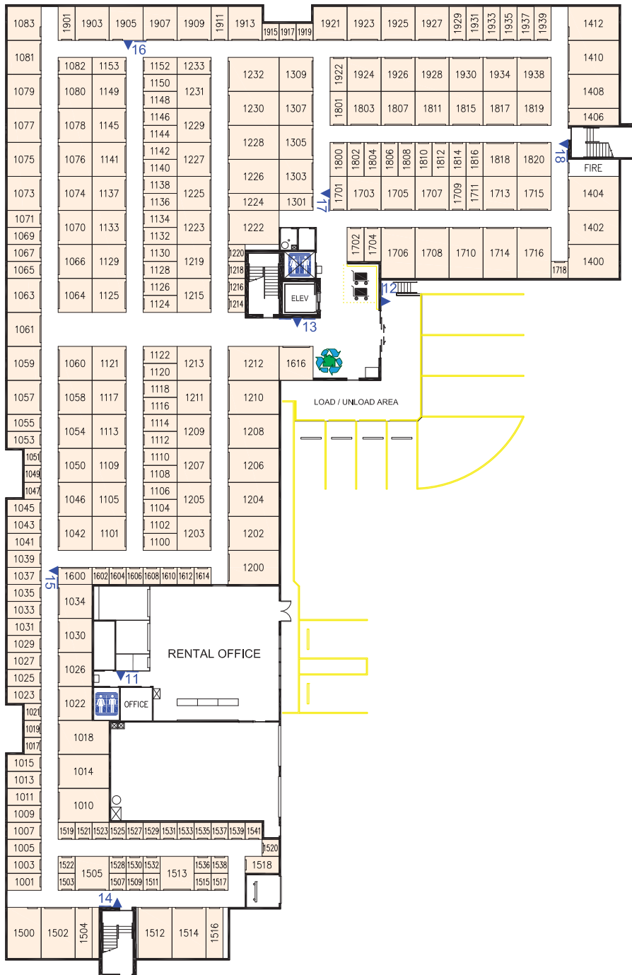
FIRST FLOOR
